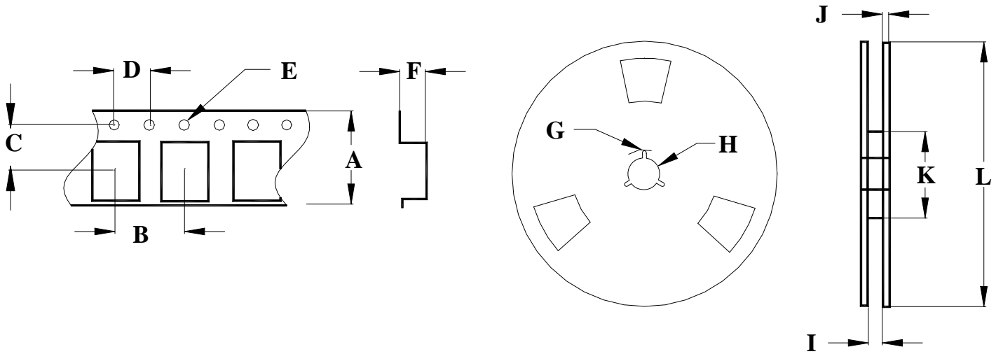
Tape and Reel Specifications for 1000 pieces. ( DIMENSIONS IN mm)
